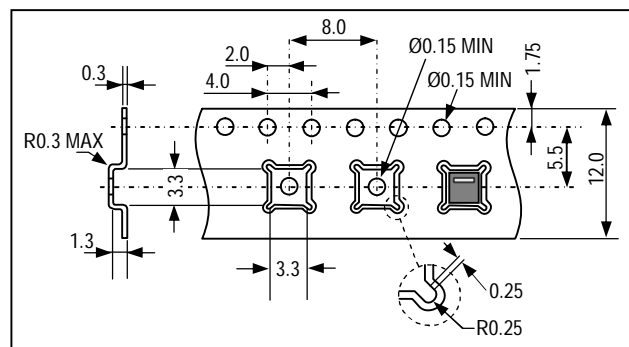
Figure 14 Sketch of packaging tape and sensor orientation.
