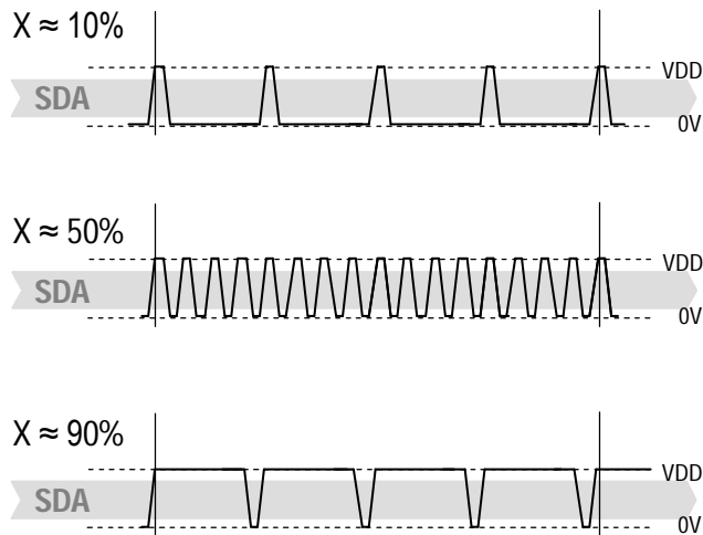
Figure 9 Schematic principle of SDM signal. X represents either RH or T at different levels of sensor output.
